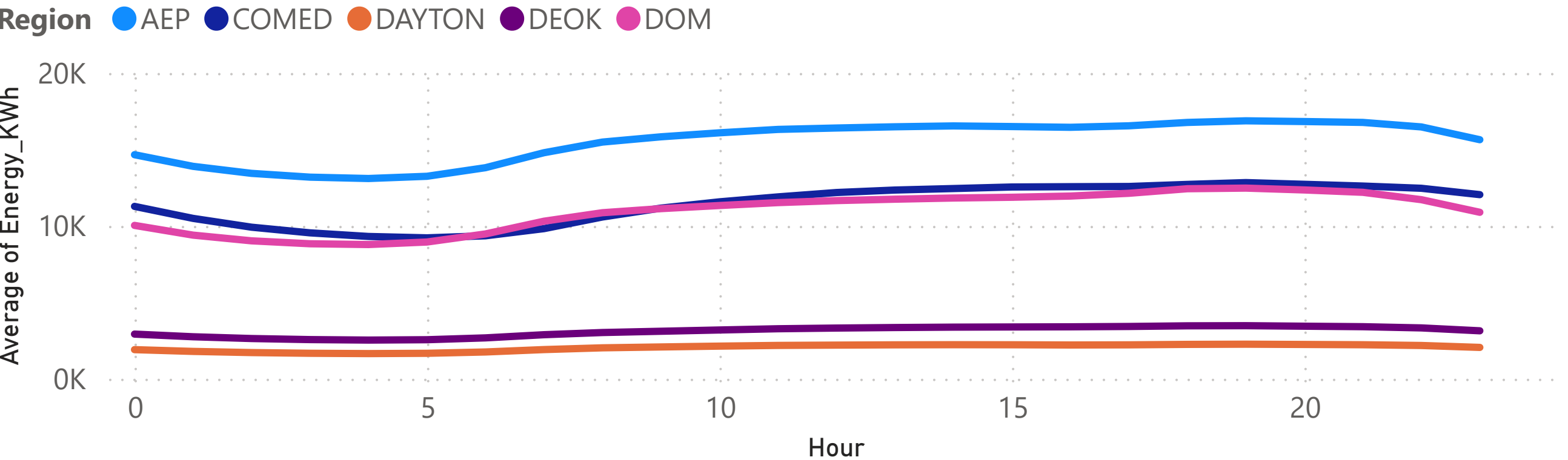
Hourly Load Profile (Line Chart)
